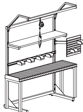
In-line Conveyor Station
